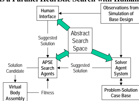
Figure 3. DBDS Performs a Parallel Heuristic Search with Human and Case-Based Guidance
