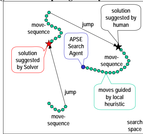
Fig. 4. Agents move and jump through the search space guided by local heuristic, human input, and case knowledge
